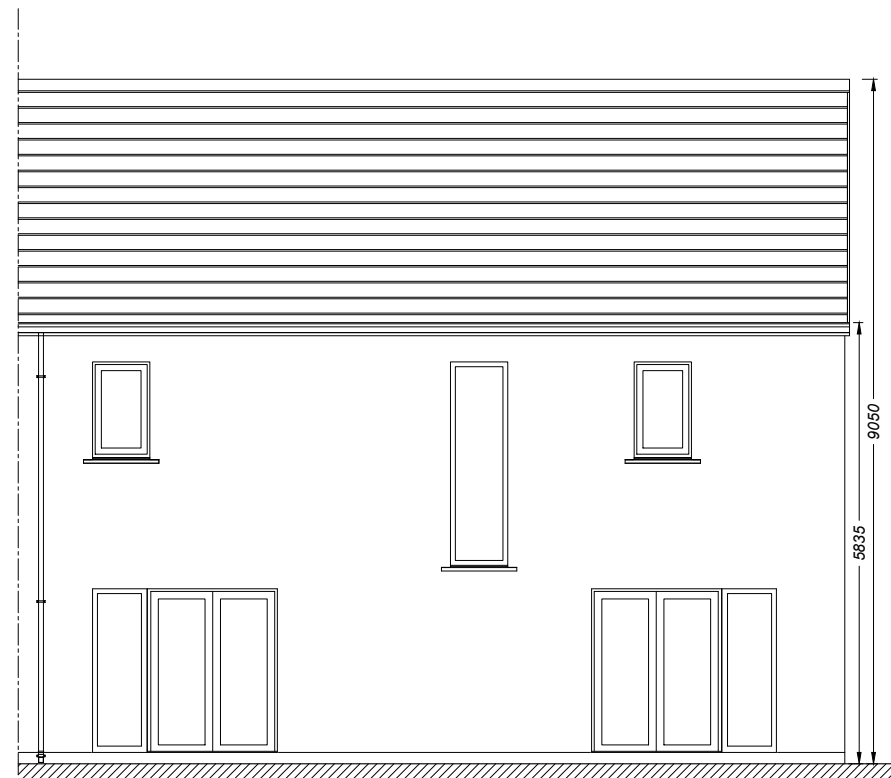
HOUSE TYPE: E REAR ELEVATION
