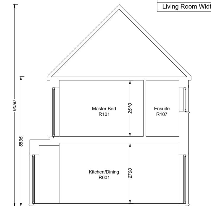
HOUSE TYPE: E SECTION AA
