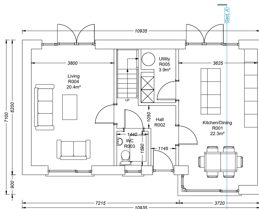
HOUSE TYPE: E GROUND FLOOR PLAN - 58.7M 2
