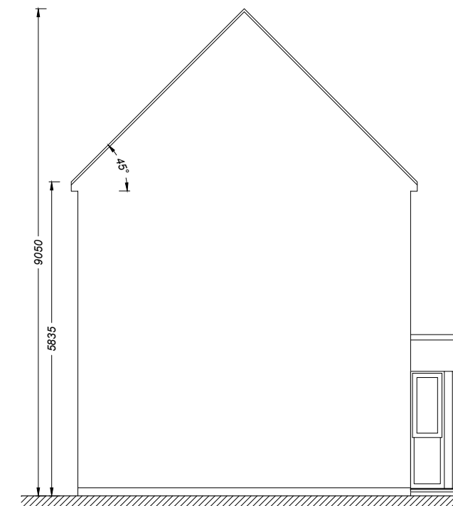
HOUSE TYPE: E SIDE ELEVATION
