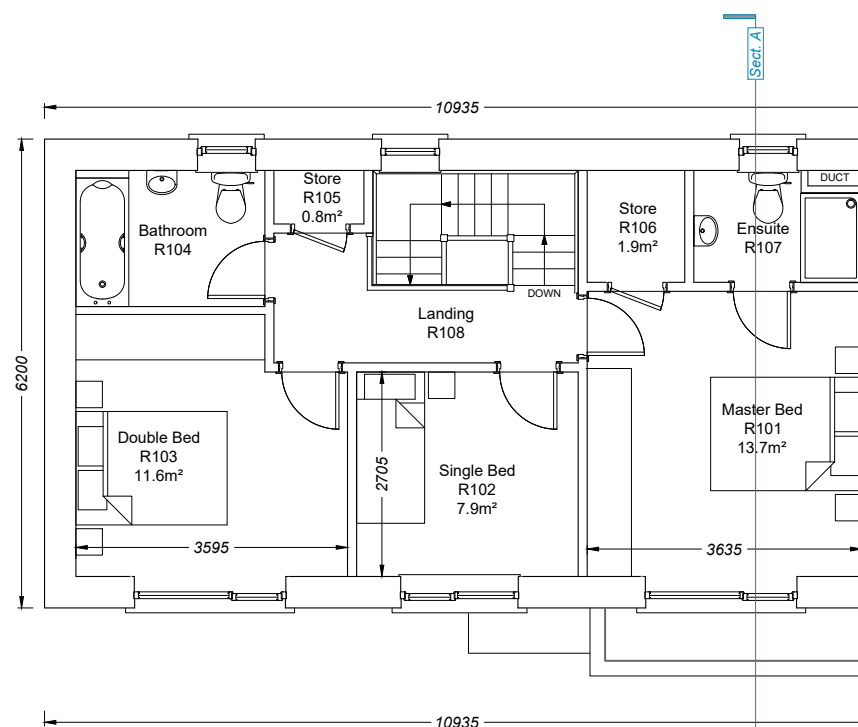
HOUSE TYPE: E FIRST FLOOR PLAN - 55.8M 2
