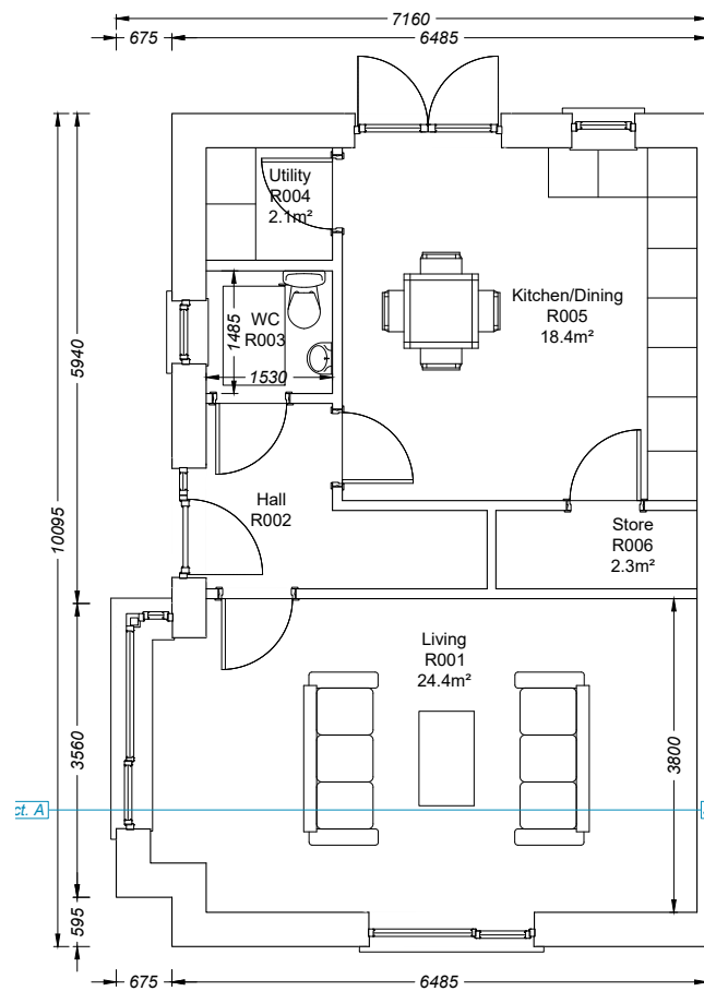
HOUSE TYPE: G GROUND FLOOR PLAN - 57.0M 2
