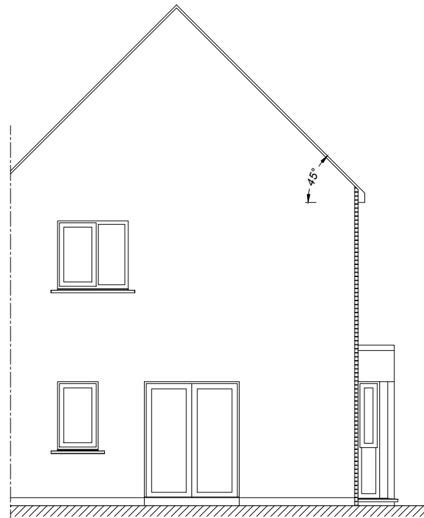
HOUSE TYPE: G REAR ELEVATION
