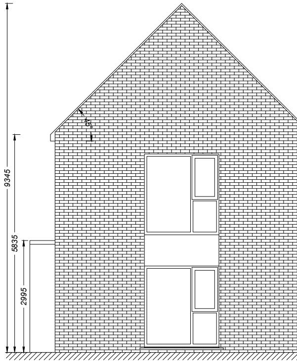
HOUSE TYPE: G FRONT ELEVATION
