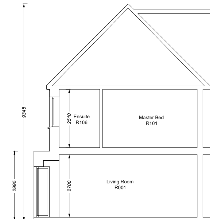
HOUSE TYPE: G SECTION AA
