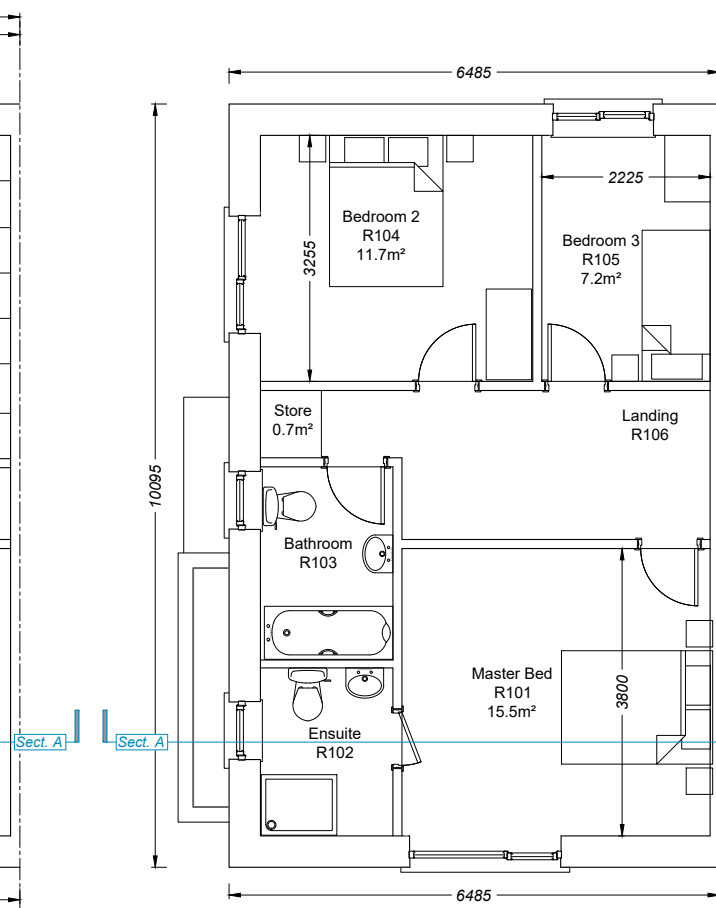
HOUSE TYPE: G FIRST FLOOR PLAN - 55.1M 2
